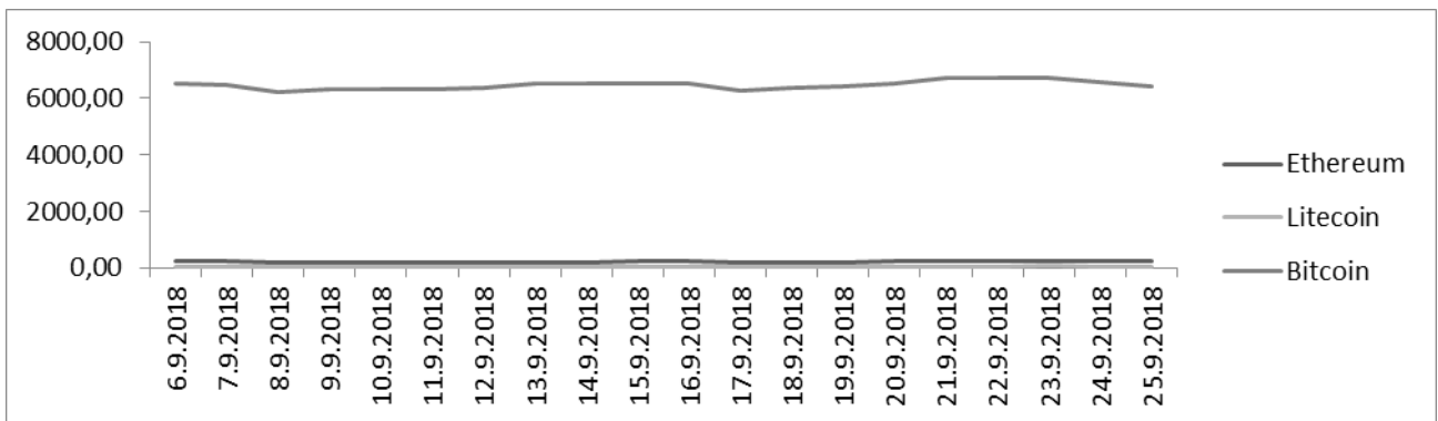
Figure 2. Cryptocurrency value in US dollars on short time periods, 4 samples of 20 observations
