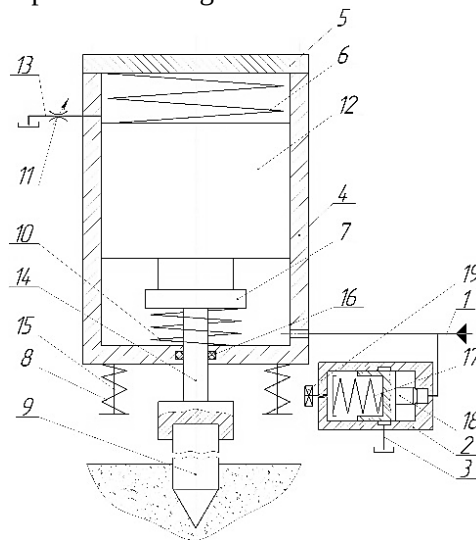
Fig. 11. Schematic diagram of a hydraulic hammer with a single-stage vibration exciter
