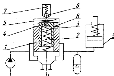
Fig. 6. Diagram of a hydraulic vibration drive with a pulsator valve: 1 – valve of the second stage 2 – spring; 3 – pusher; 4 – throttle hole; 5 – supravallular cavity; 6 – ball; 7 – spring; 8 – spring; 9 – cylinder cavity
