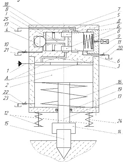
Fig. 10. Schematic diagram of a hydraulic hammer with a built-in vibration exciter
