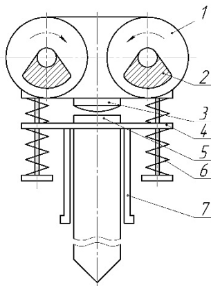
Fig. 3. Schematic diagram of a vibrating hammer
